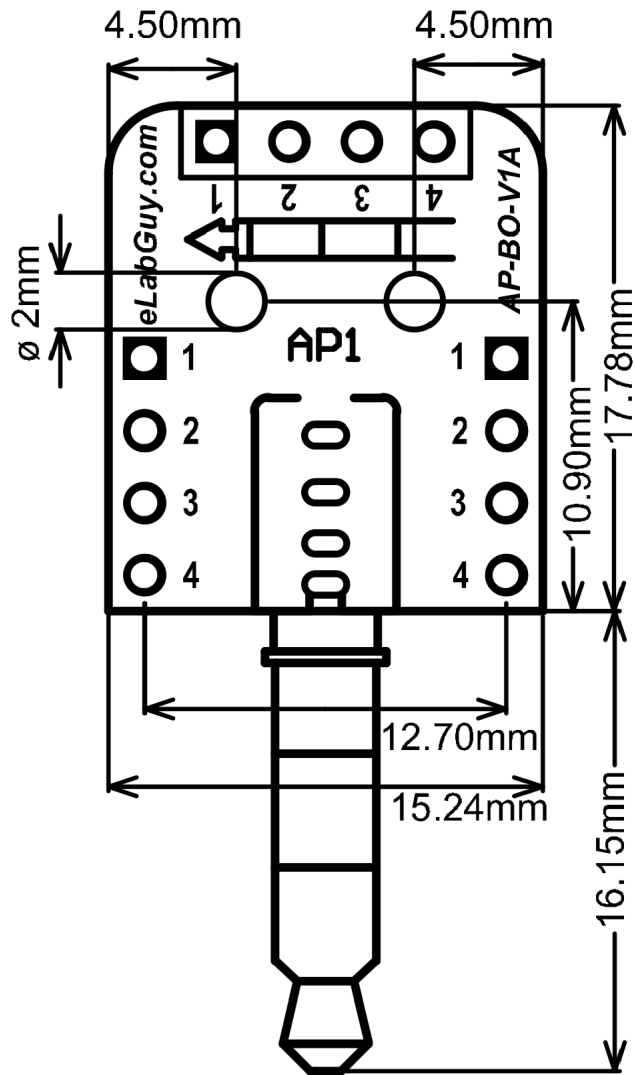
AP-BO-V1A PCB outline Drawing
