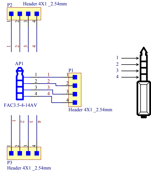
AP-BO-V1A Schematic Diagram
